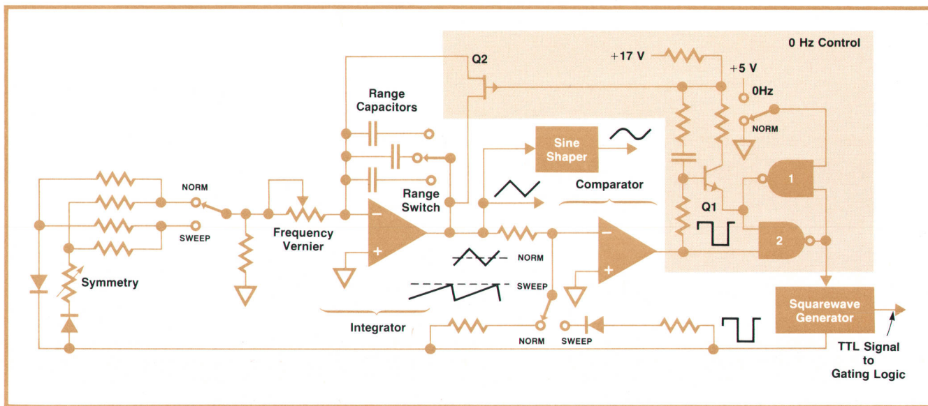
Fig. 7. Modulation generator uses an integrator for very low frequency operation. Reset level and symmetry are altered for ramp waveforms.
