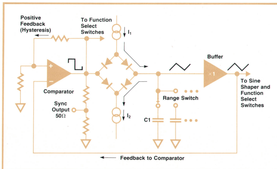
Fig. 6. Main generator produces triangle waves and square waves as part of its normal operation. The square wave is divided down to 1 volt peak for the sync output. Asymmetrical control of currents I_1 and I_2 provides a means of varying the up-down ratio of the triangle (see box on opposite page).
